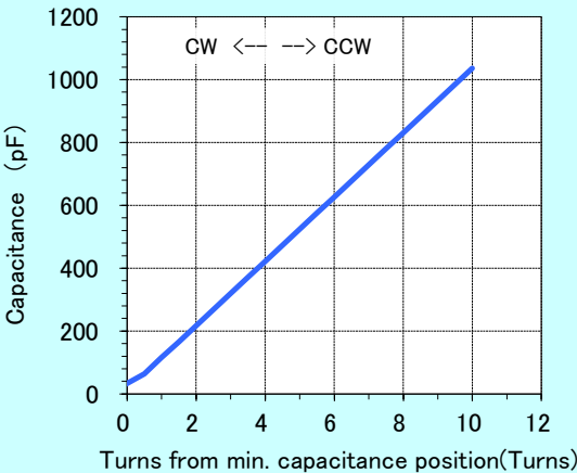
Tuner Turns – Capacitance response
