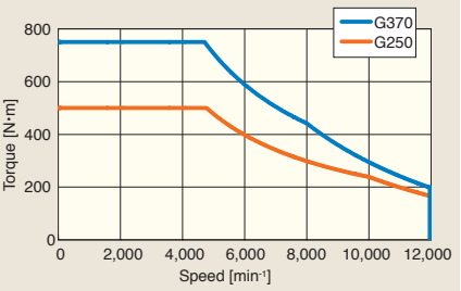
Torque curve (Absorbing)
