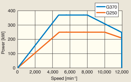
Power curve (Absorbing)
